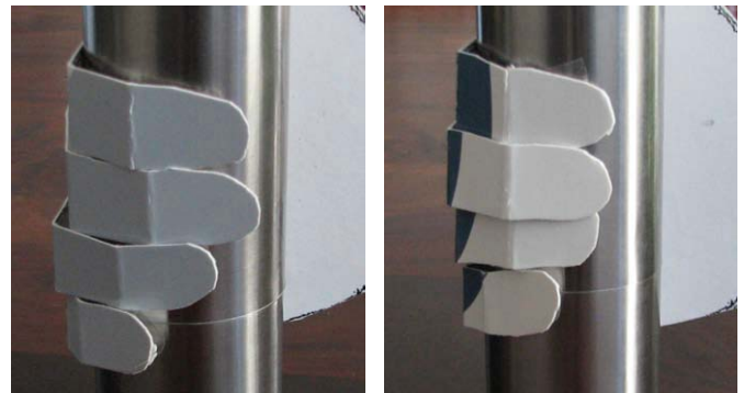
Fig. 11. Testing inclination of PIP and DIP joints performing power grasp on a pepper mill. The used prototypes have no mobility within the thumb and the metacarpal joints of the fingers and are fixed using tape for visualization purpose which is not optimal for positioning of the fingers).
